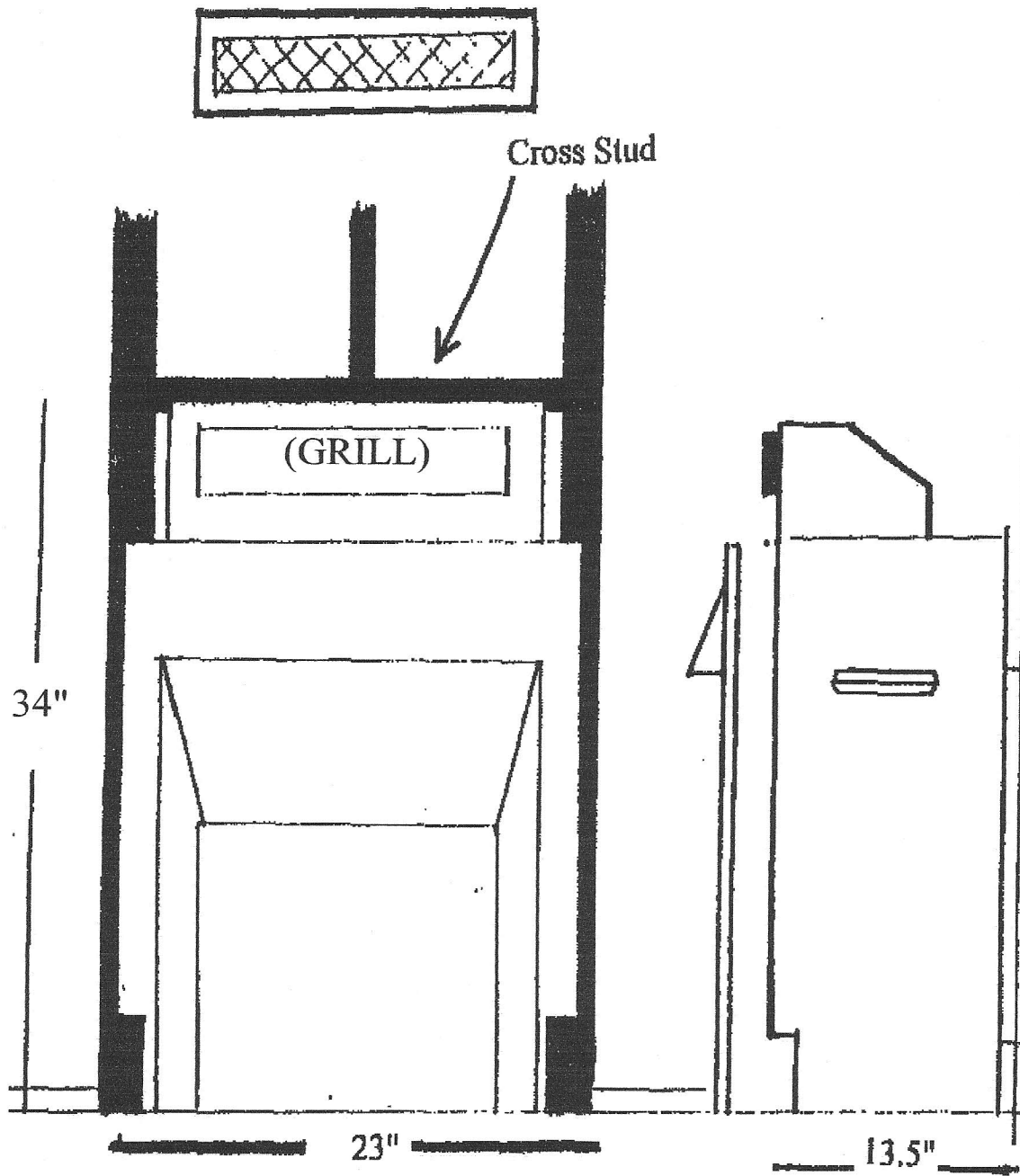
Front View : Cross stud support behind vent flange.
