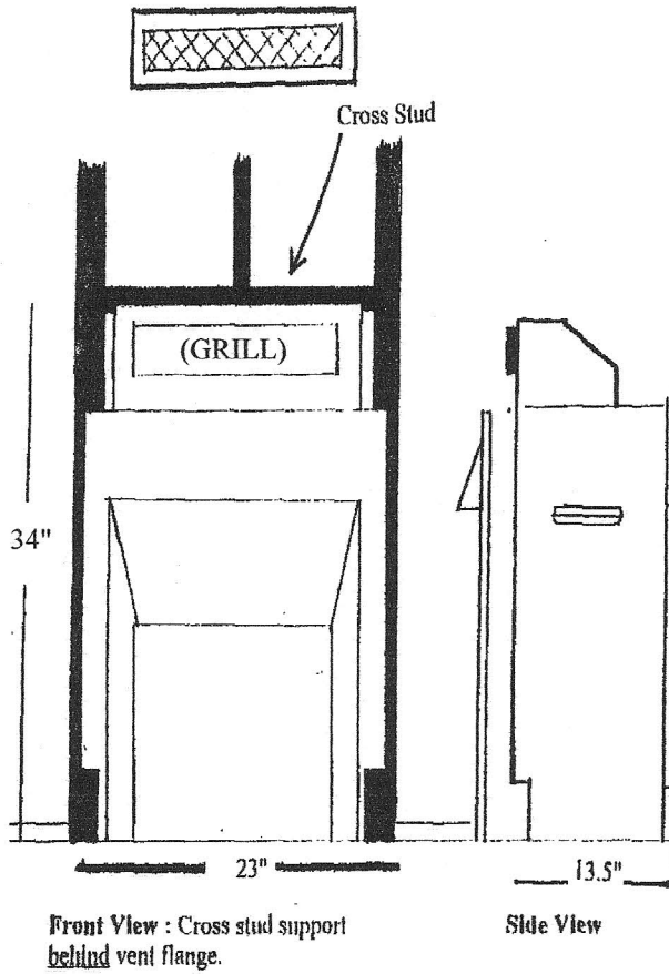
20" VENTFREE FIREBOX
